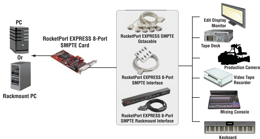
RocketPort EXPRESS 8-Port SMPTE Interface
